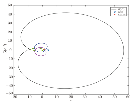
Figure 1 (Color online) The curve of G(e^{it})
