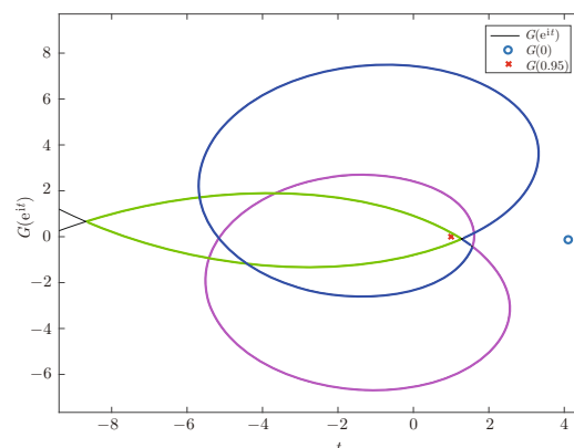
Figure 2 (Color online) Local details of G(e^{it})
